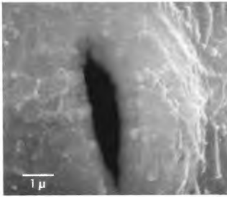
Abb. 25: Alnus glutinosa (Rezentmaterial), Apertur (Foto KNICKREHM, NLfB)
